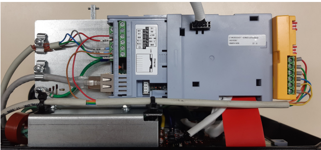
Figure A.6: Example of connection of shield and clamps of control cables
