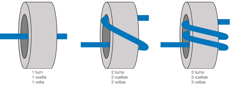
Figure B.1: Passage of the cables through the ferrite for 1, 2 and 3 turns
