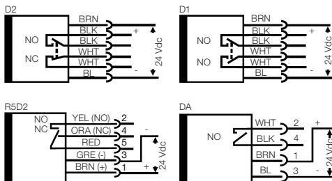
Figure 1: Electric diagram
