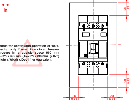
<FIG. 1> Clearance for Circuit Breaker
