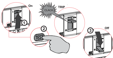
<FIG. 4> Circuit Breaker Manual controls
