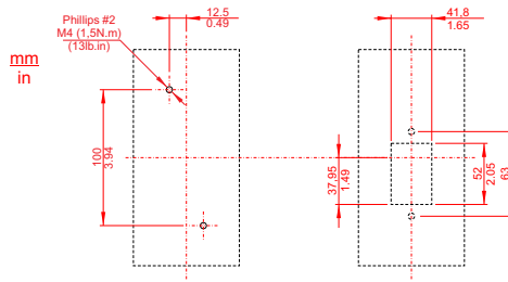
<FIG. 2> Circuit Breaker Drilling Template
