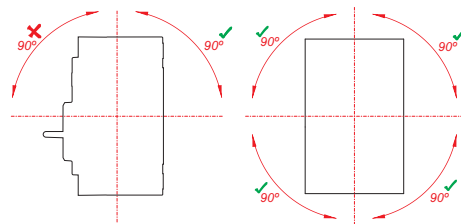
<FIG. 6> Operating Positions
