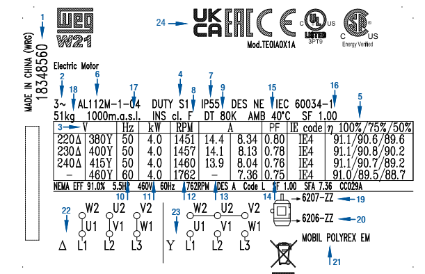
Figure 7 -Nameplate
