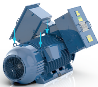
Figure 4 - Eyebolt fixing points for lifting motors with two terminal boxes.
