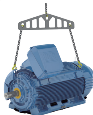
Figure 8 - Lifting with inclined chains.
