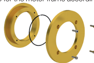
Figure 48 - Taconite Labyrinth
