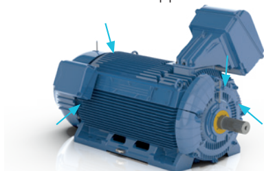
Figure 39 - Location of vibration measuring points.
