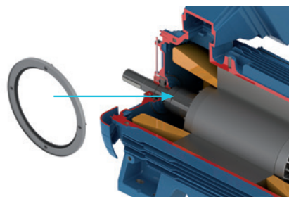
Figure 13 - AEGIS grounding ring.
