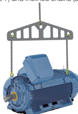
Figure 7 - Lifting with vertical chains.
