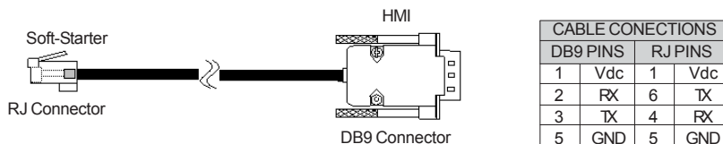
Figure 19.1 - Cable CAB-RS for HMI-SSW05-RS.
