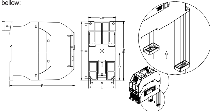
Figure 10.1 - SSW-05 Plus Dimensions
