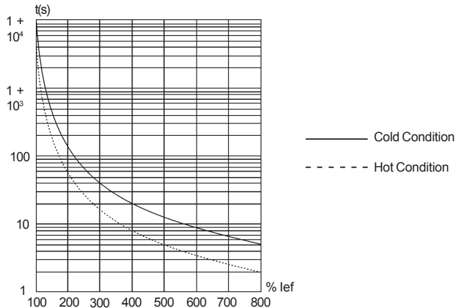
Figure 15.1 - Curve of the motor electronic overload protection.
