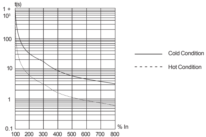
Figure 15.2 - Curve of the thyristor overload.
