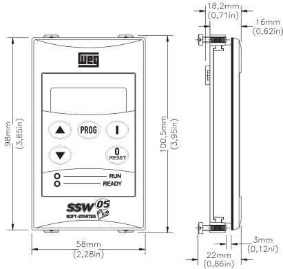
Figure 19.3 - Dimensions of the HMI-SSW05-RS.
