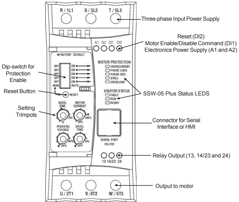
Figure 5.1 - SSW05 Plus Front view
