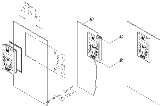
Figure 19.5 - HMI-SSW05-RS Installation.
