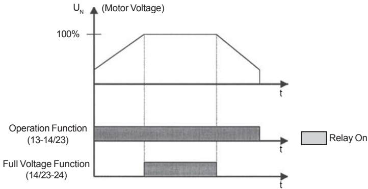
Figure 13 - Operation of the digital relay outputs.
