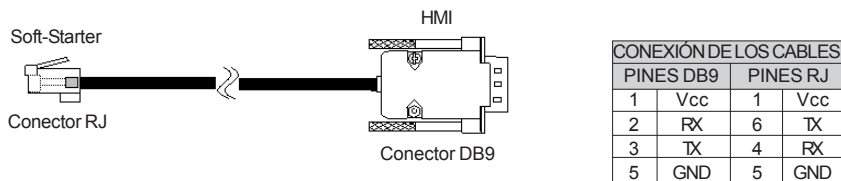
Figura 19.1- Cable CAB-RS para HMI-SSW05-RS
