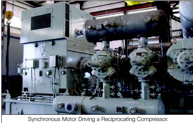
Synchronous Motor Driving a Reciprocating Compressor.
