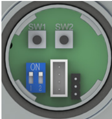
Figure 8 - Product standard control switches
