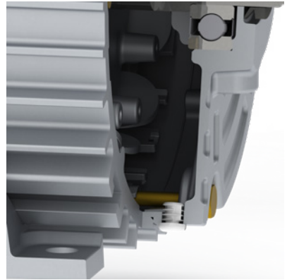
Figure 6 - Drain sectional
