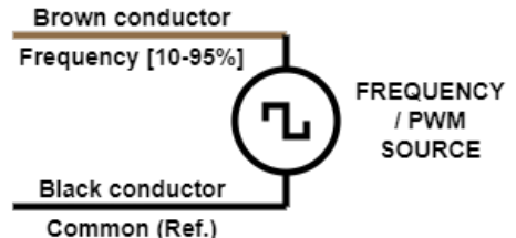
Figure 12 - Frequency input
