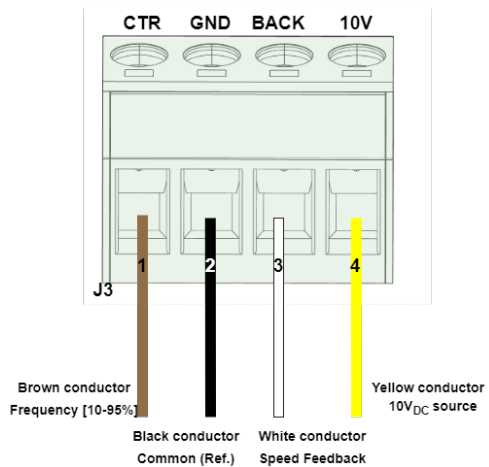
Figure 14 - Controller sequence connection
