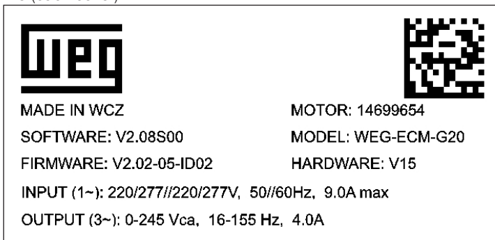
Figure 1 - Drive label
