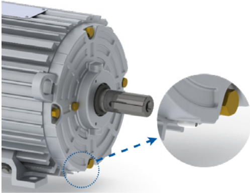
Figure 5 - Drain position
