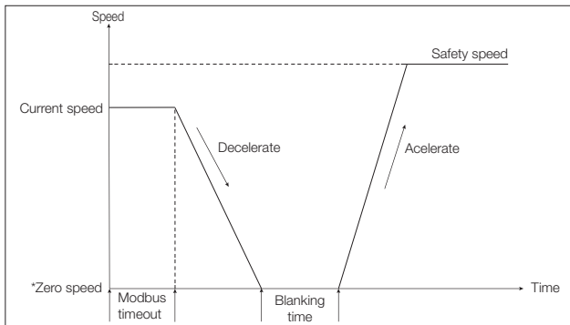
Figure 15 - Time out logic for s04 firmware version
