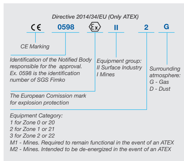
ATEX marking
