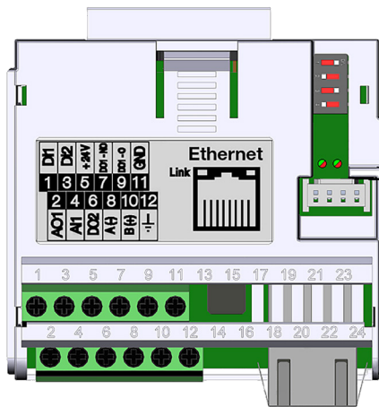
图 20.5: CFW500-CEMB-TCP / CFW500-CETH-IP / CFW500-CEPN-IO 插件模块
