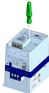
(f) Tighten the screws of the accessory (Torque: 0.51 N/m) (f) Apriete los tornillos del accesorio (Torque: 0.51 N/m) (f) Aperte os parafusos do acessório (Torque: 0.51 N/m)
