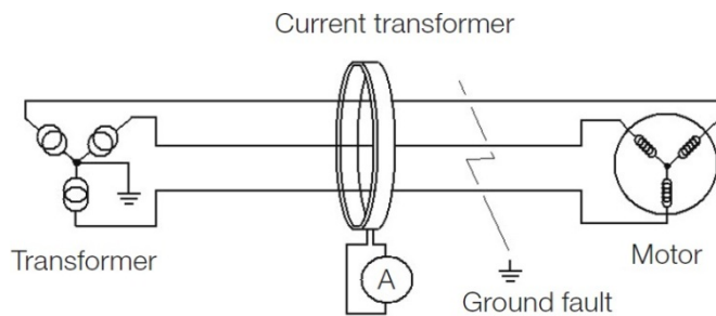
Figure 1 – Ground fault protection by measurement of leakage current.
