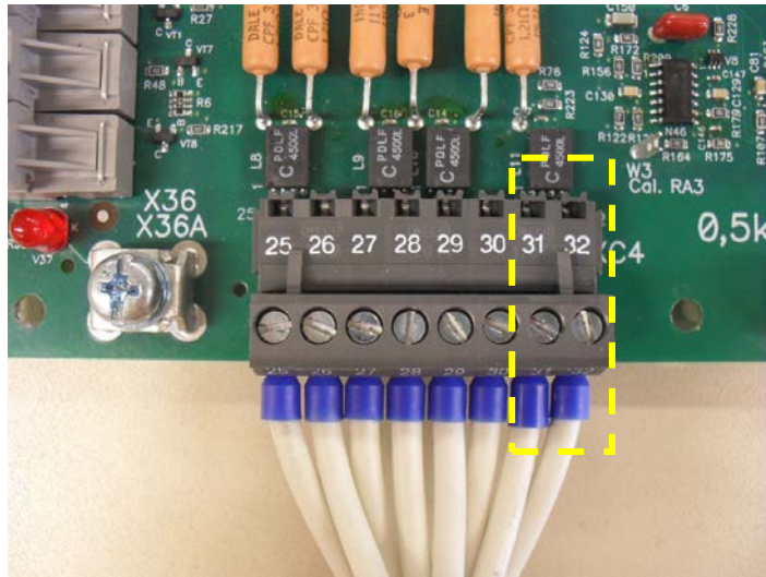
Figure 5 – Connection of the ground fault CT to the CSMx card
