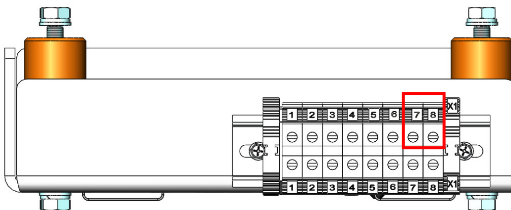
Figure 4: Terminals (7 and 8) to connect the cables of the ground fault CT.
