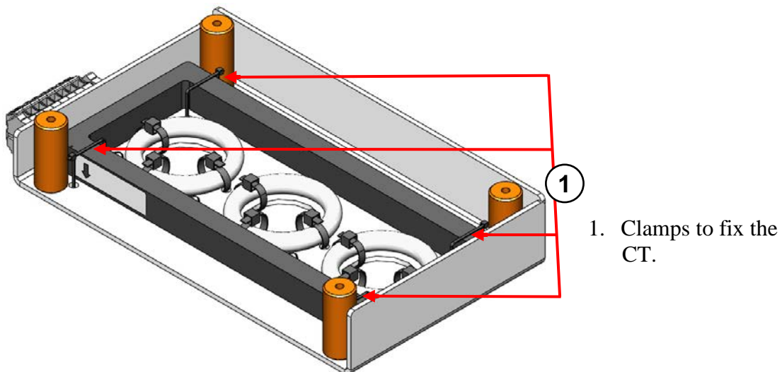
Figure 2: Installation of the ground fault CT.
