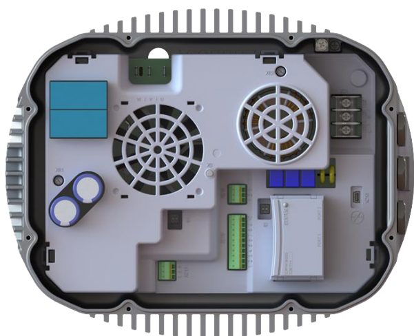
Figure 6 - Drive view
