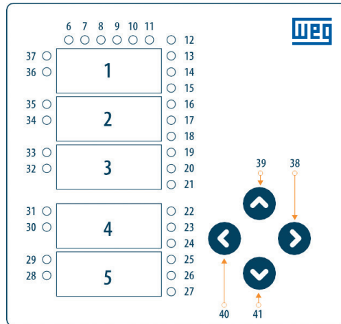
Figura 1.1: MMW03-CH Front Panel
