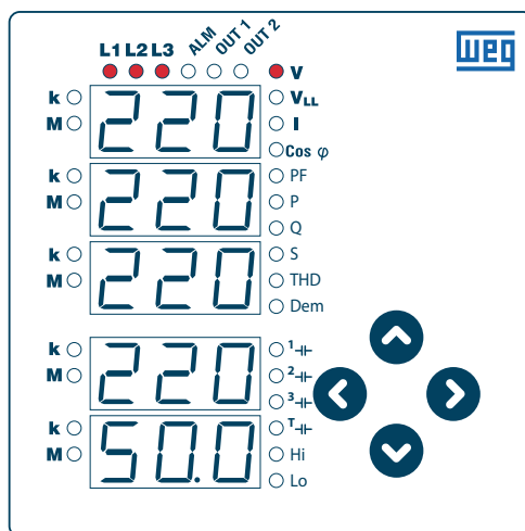
Figura 3.1: Voltage (Phase-Neutral) Display
