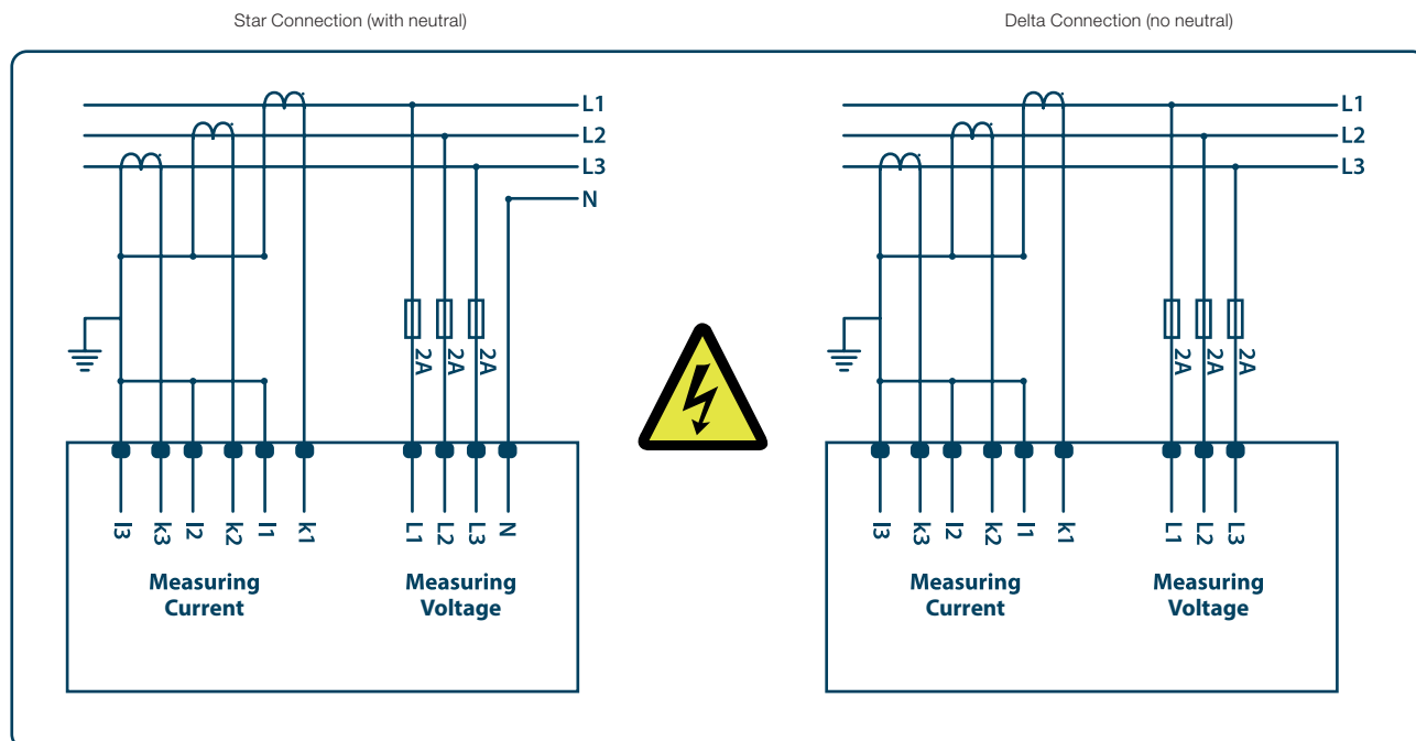
Figura 2.1: Connection Diagram
