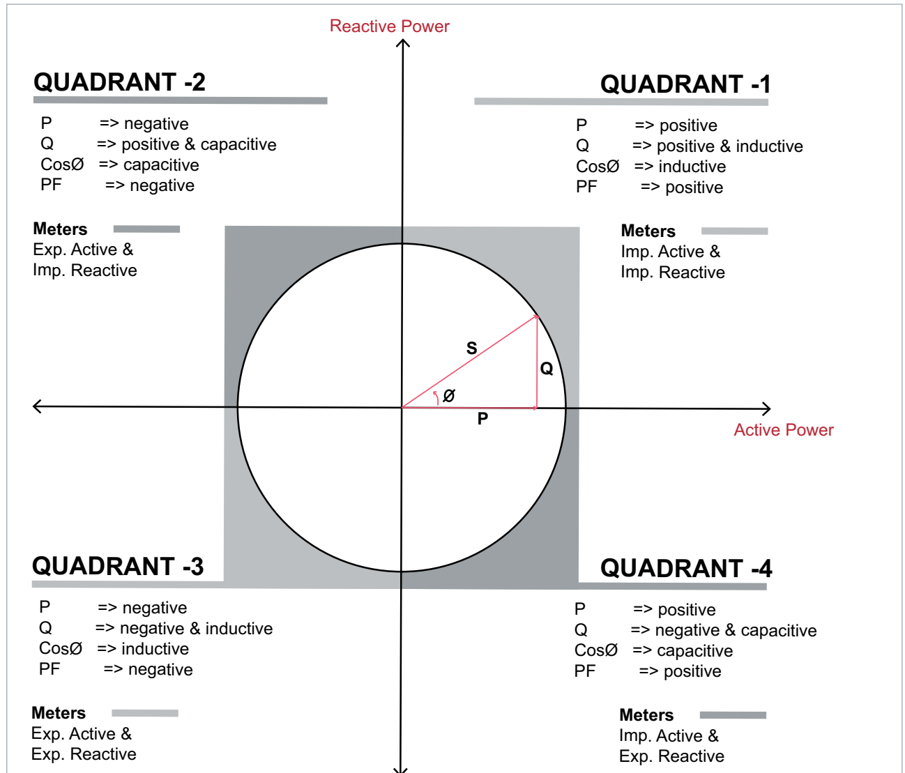
Figura 1.2: Four Quadrant Representation
