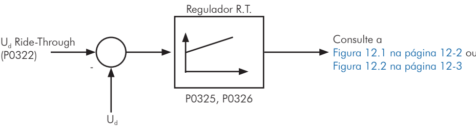
Figura 12.3 - Controlador PI do Ride-Through
