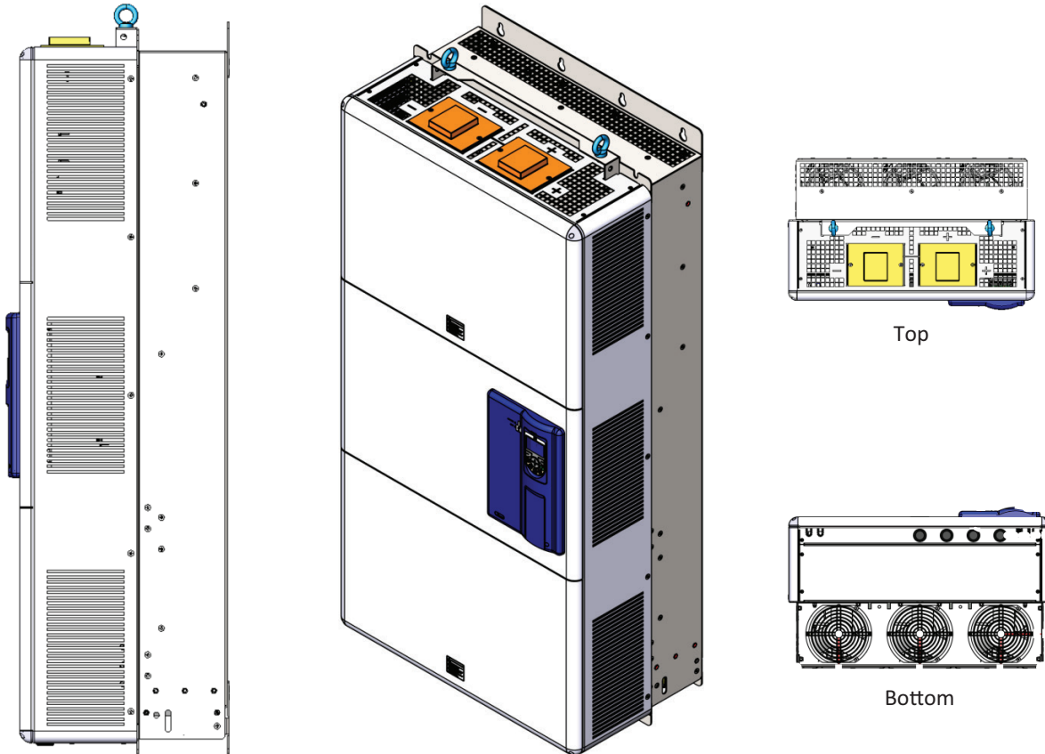
CFW11 Frame H Drive Module
